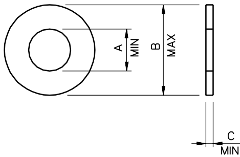
WASHER
