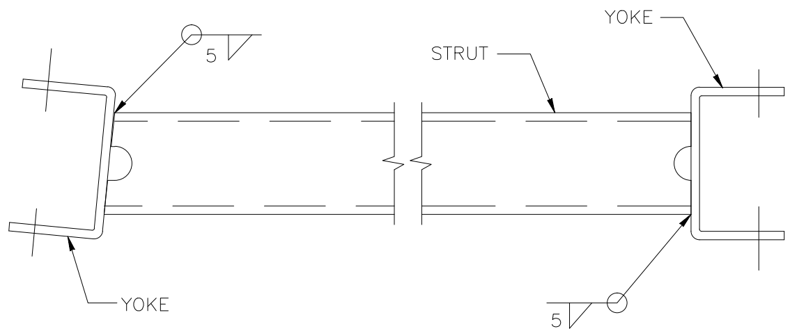
ASSEMBLY DETAILS
