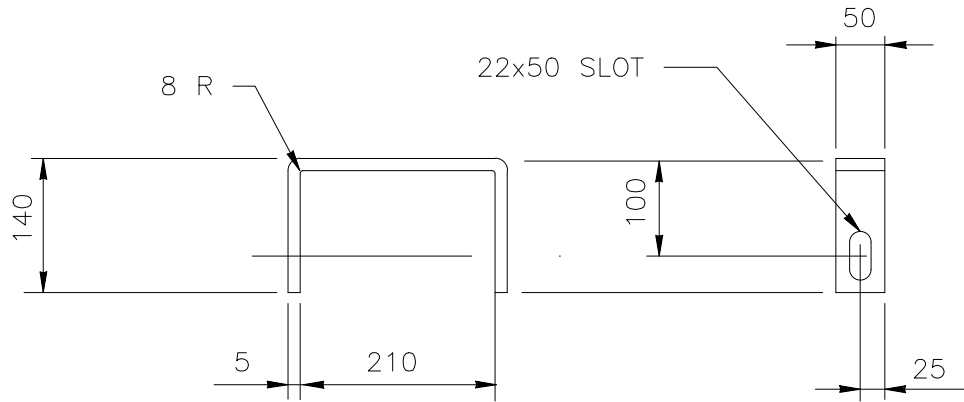
YOKE DETAILS (2 REQUIRED)
