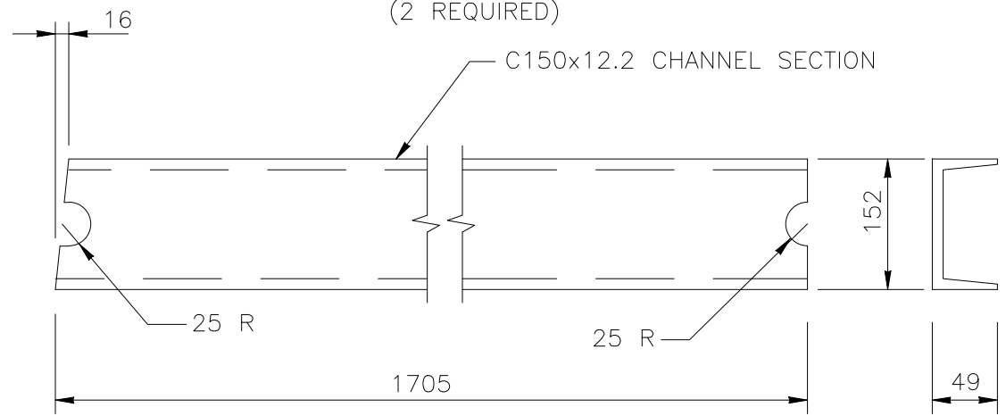
STRUT DETAILS
