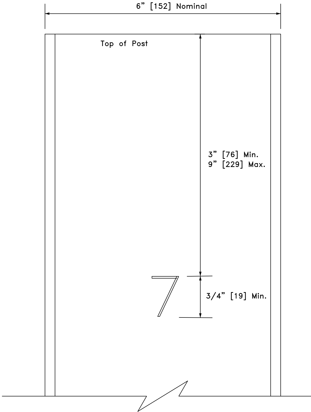
SIDE VIEW
