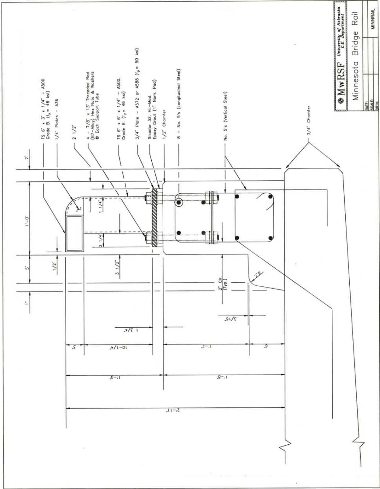
Figure 1. Minnesota Combination Bridge Rail Design Details, Design No. 1.
