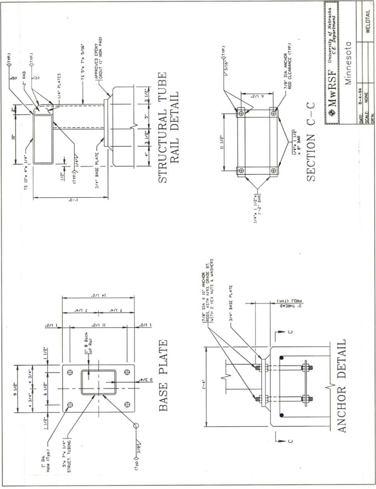
Figure 9. Minnesota Combination Bridge Rail Details, Design No. 3.
