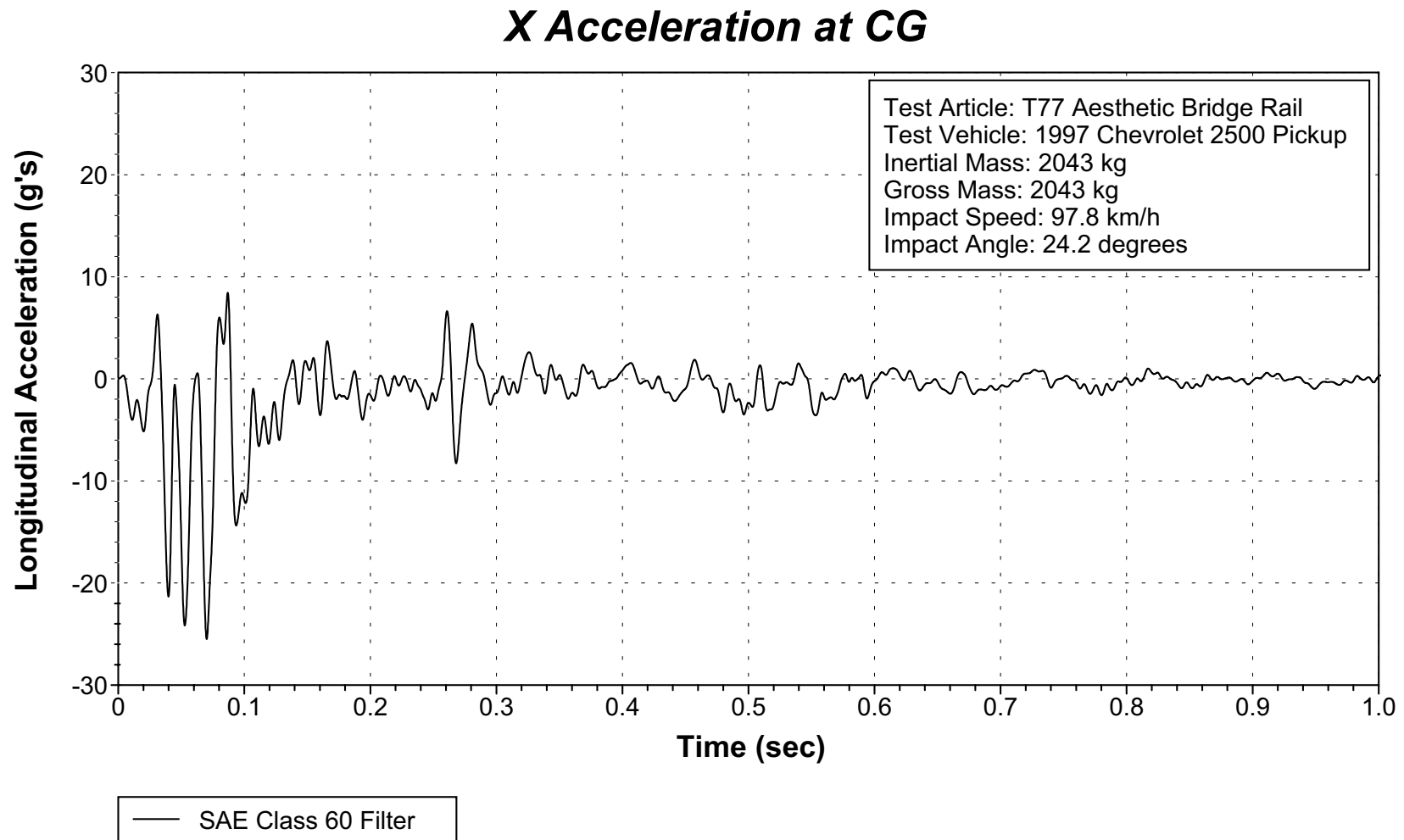
Figure 62. Vehicle Longitudinal Accelerometer Trace for Test 442882-3 (Accelerometer Located at Center of Gravity).
