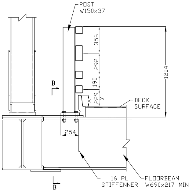
SECTION
