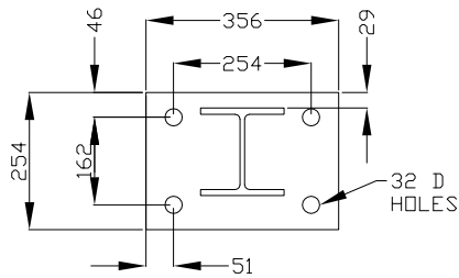
POST & BASE PLATE PLAN
