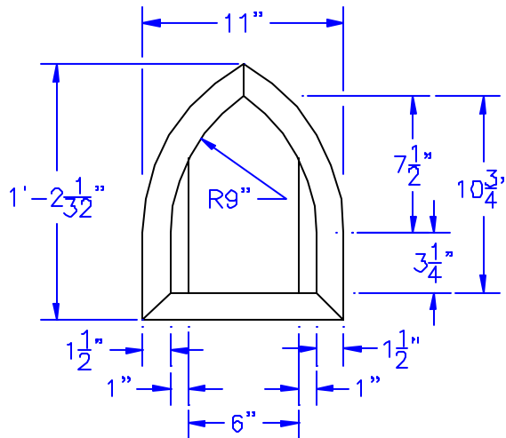
DETAIL 1 ~ WINDOW DETAILS
