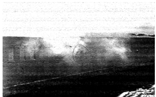
Figure 39. Sequential Photographs for Test 442882-1 (Rear View).
