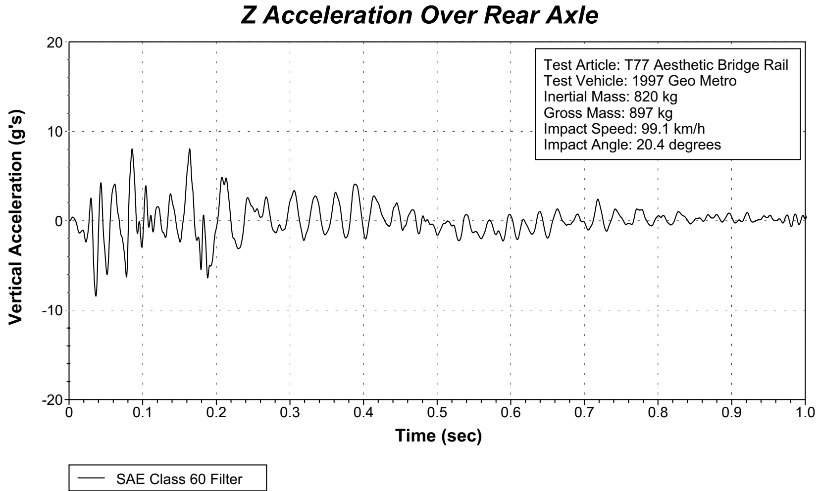
Figure 73. Vehicle Vertical Accelerometer Trace for Test 442882-4 (Accelerometer Located Over Rear Axle).
