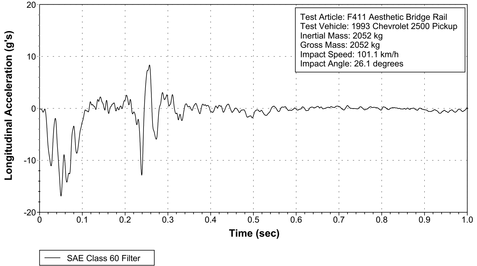
Figure 59. Vehicle Longitudinal Accelerometer Trace for Test 442882-2 (Accelerometer Located Over Rear Axle).
