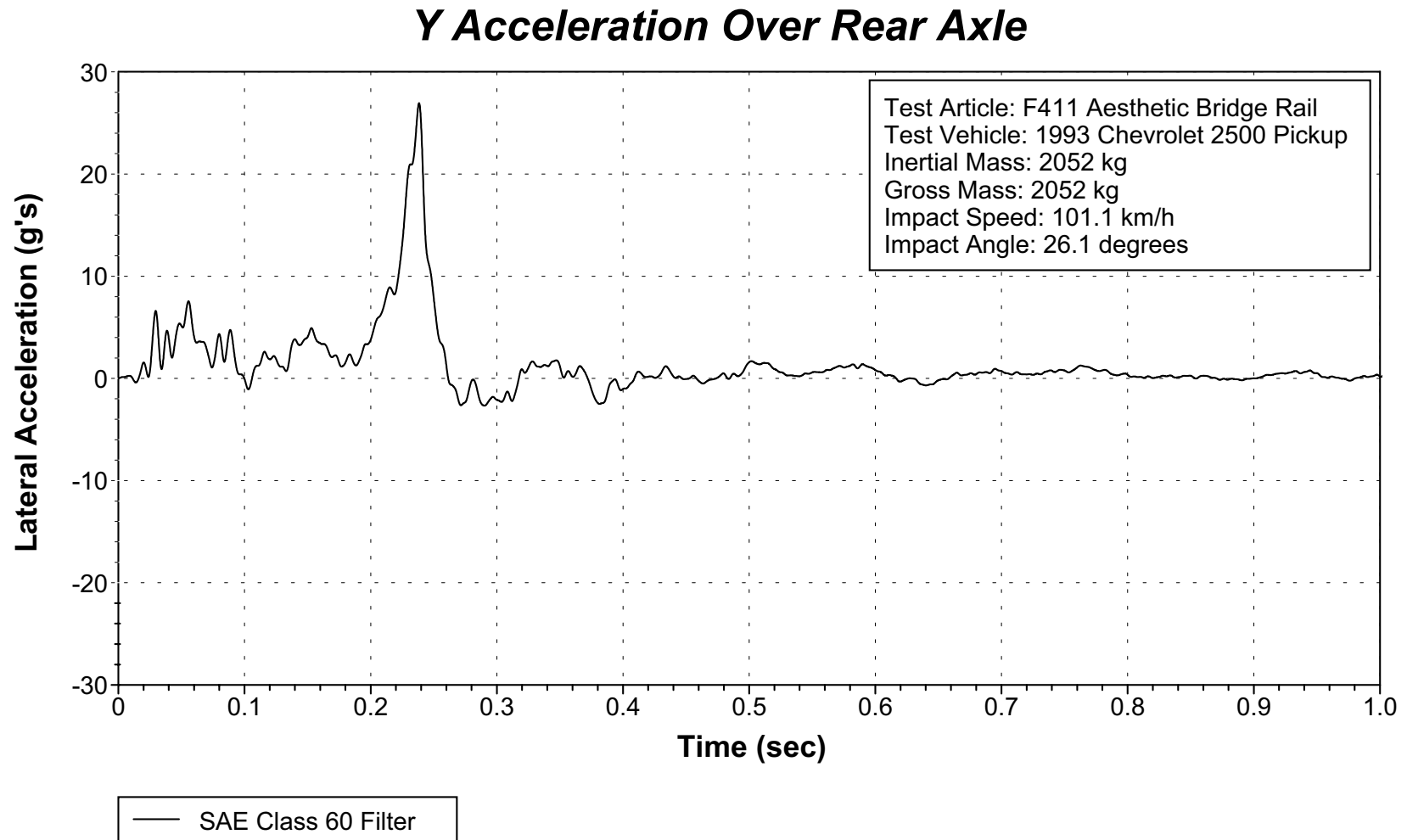
Figure 60. Vehicle Lateral Accelerometer Trace for Test 442882-2 (Accelerometer Located Over Rear Axle).
