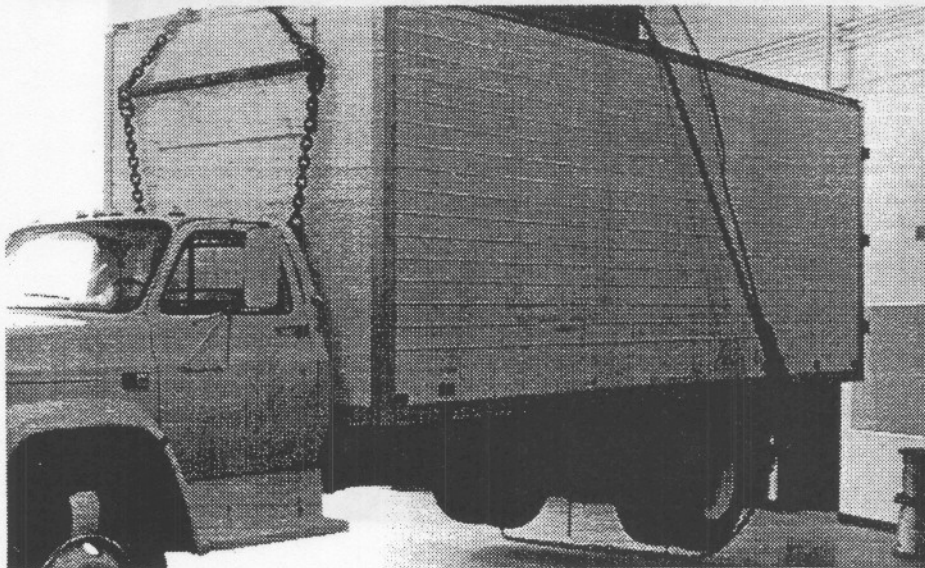
Figure 13. Photographs of center-of-mass determination using suspension method.
