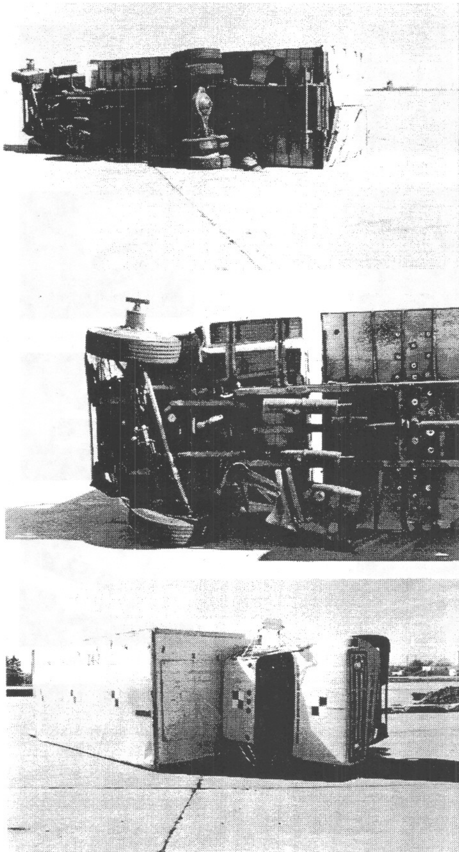
Figure 25. Photographs of vehicle damage, Test I4-2.
