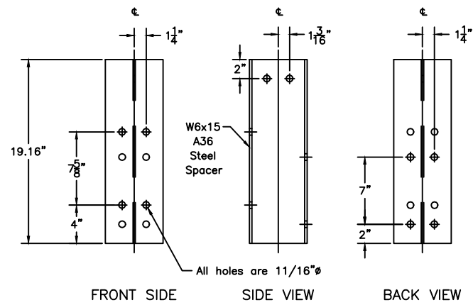
Spacer Block
