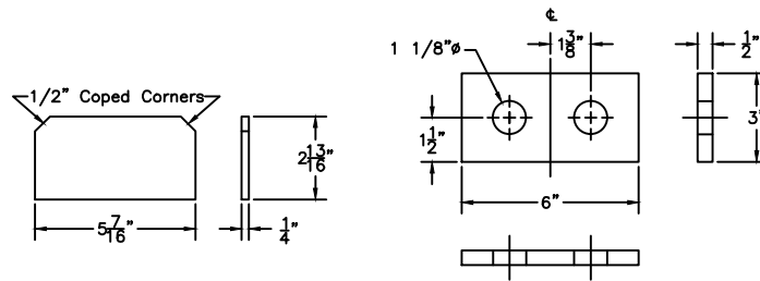
Post Stiffener
