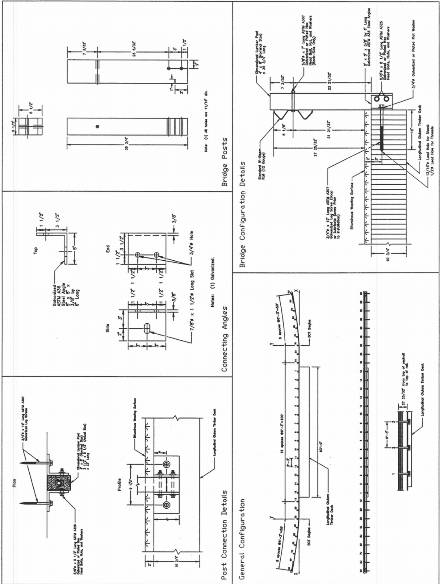
Figure 26. Flexible W-Beam Bridge Railing System Design Details, Design No. 2
