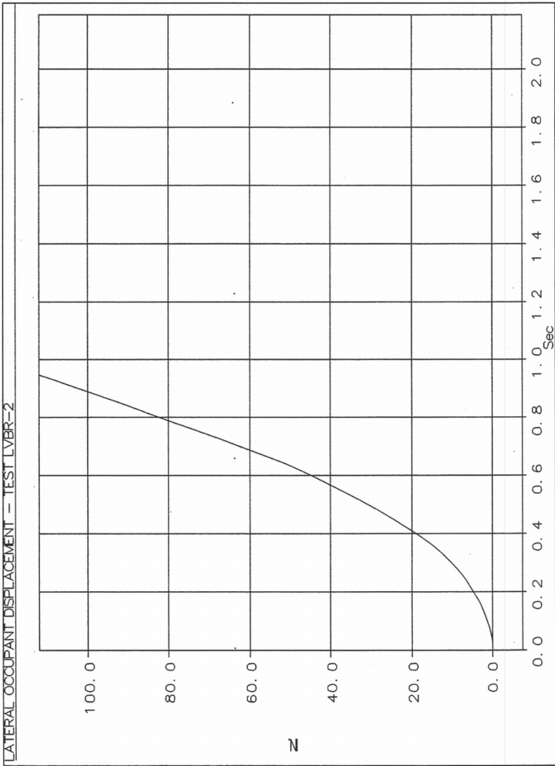
Figure A-12. Graph of Lateral Occupant Displacement, Test LVBR-2
