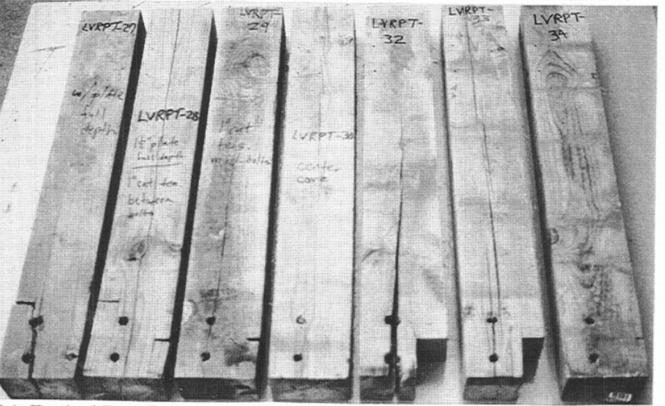
Figure 24. Typical Post Failures
