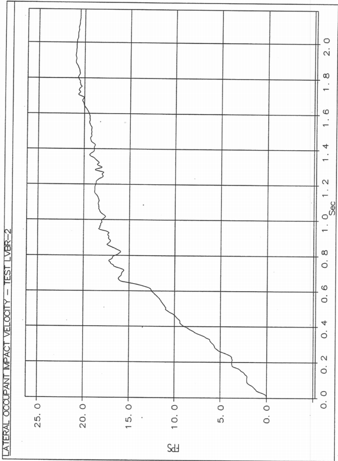
Figure A-11. Graph of Lateral Occupant Impact Velocity, Test LVBR-2
