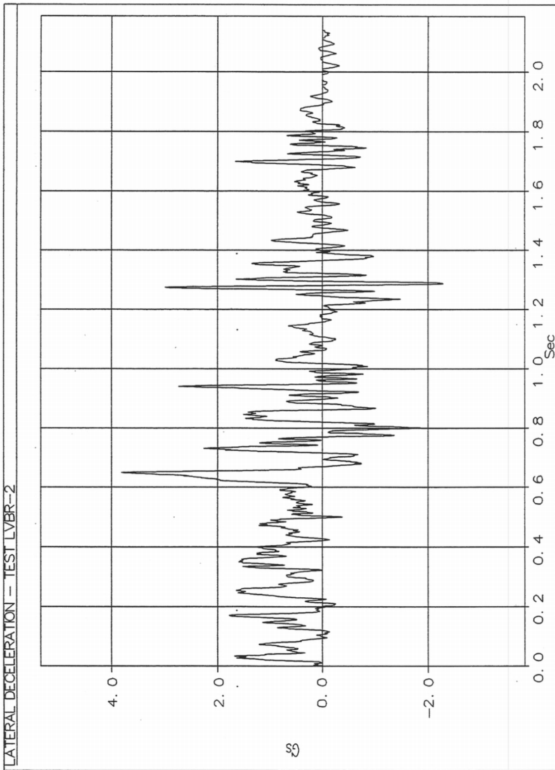
Figure A-10. Graph of Lateral Deceleration, Test LVBR-2
