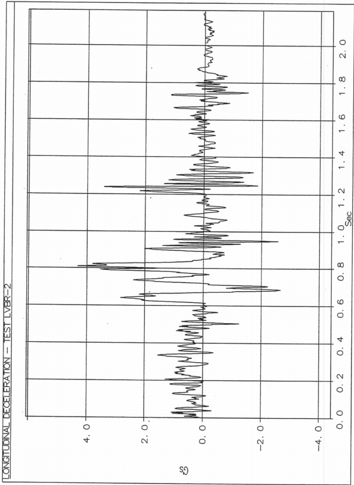
Figure A-7. Graph of Longitudinal Deceleration, Test LVBR-2
