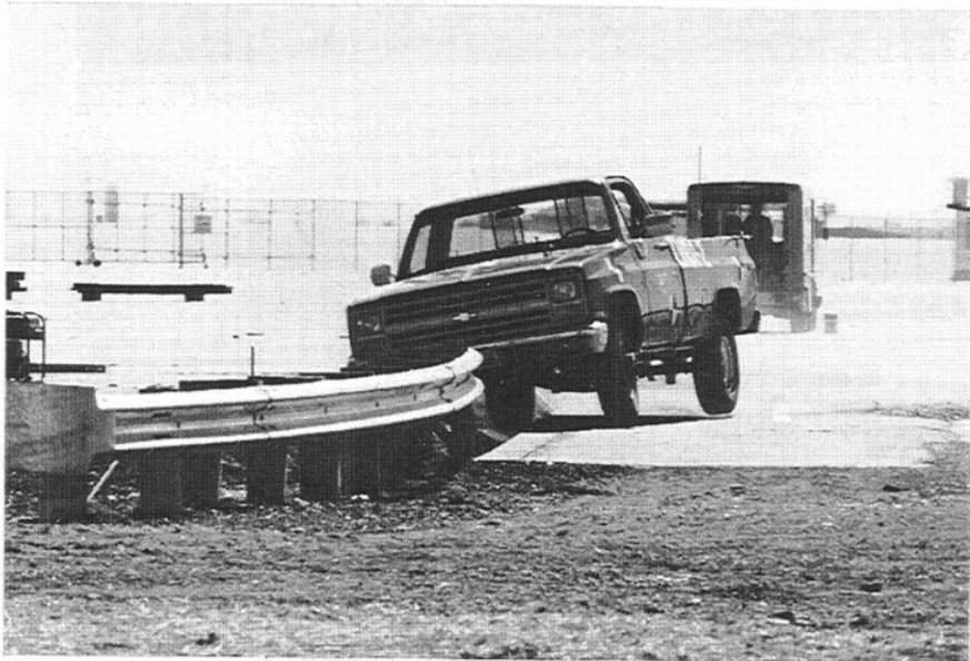
Figure 30. Documentary Photographs, Test LVBR-2
