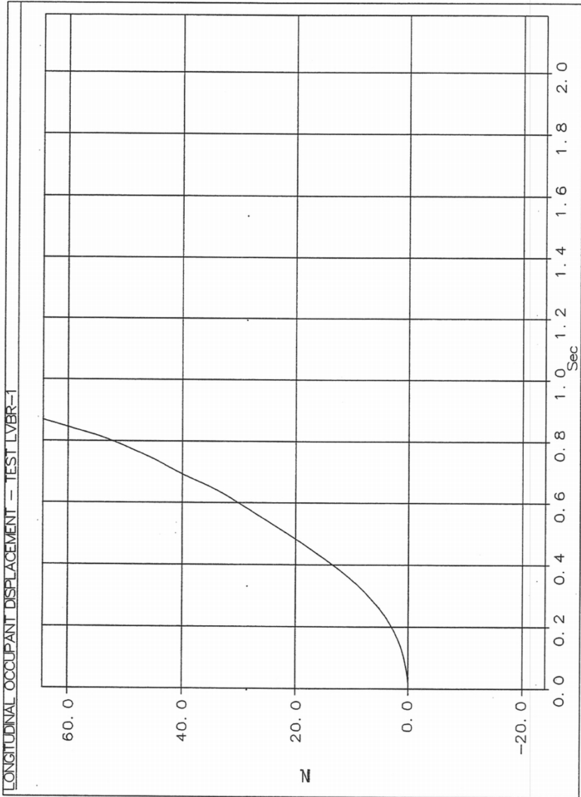
Figure A-9. Graph of Longitudinal Occupant Displacement, Test LVBR-2
