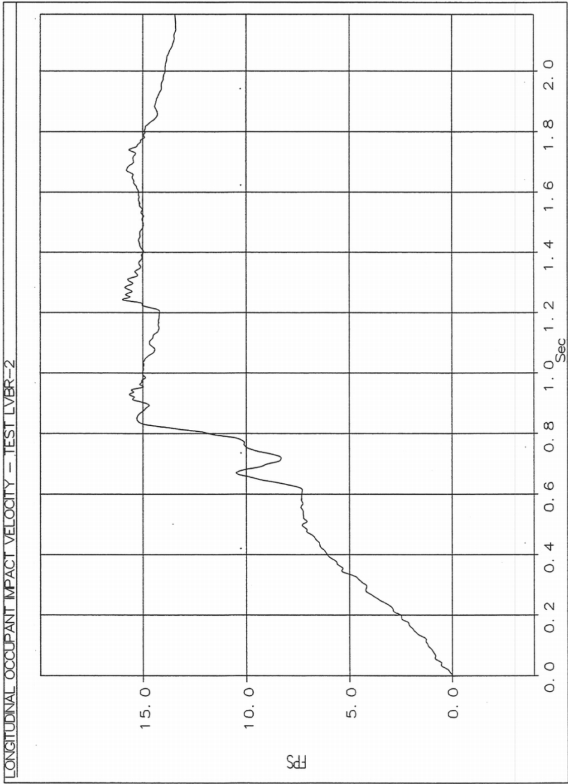
Figure A-8. Graph of Longitudinal Occupant Impact Velocity, Test LVBR-2
