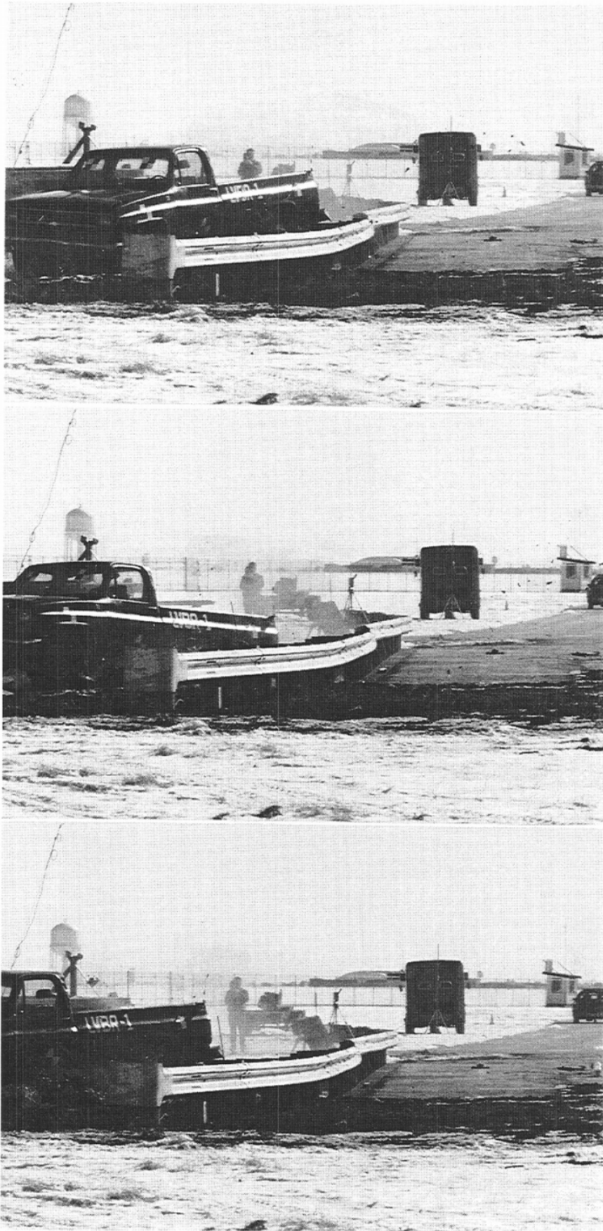
Figure 18. Documentary Photographs, Test LVBR-1
