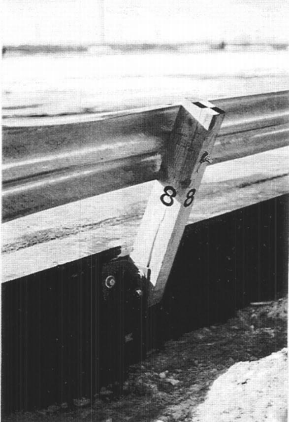
Figure 22. Bridge Post Damage, Test LVBR-1
