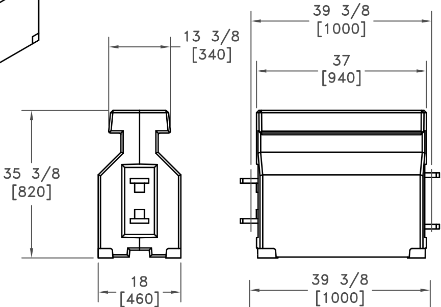
CONCRETE REACTIVE TENSION® BARRIER
