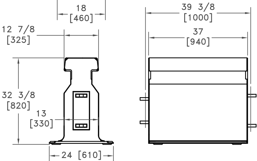
STEEL SHELL REACTIVE TENSION® BARRIER
