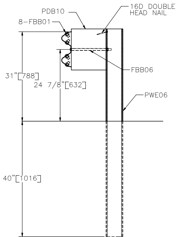
SGR21a Section A-A
