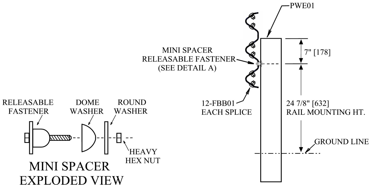
DETAIL A
