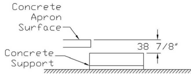
ELEVATION VIEW
