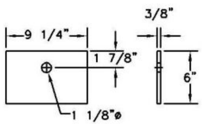
End Plates
