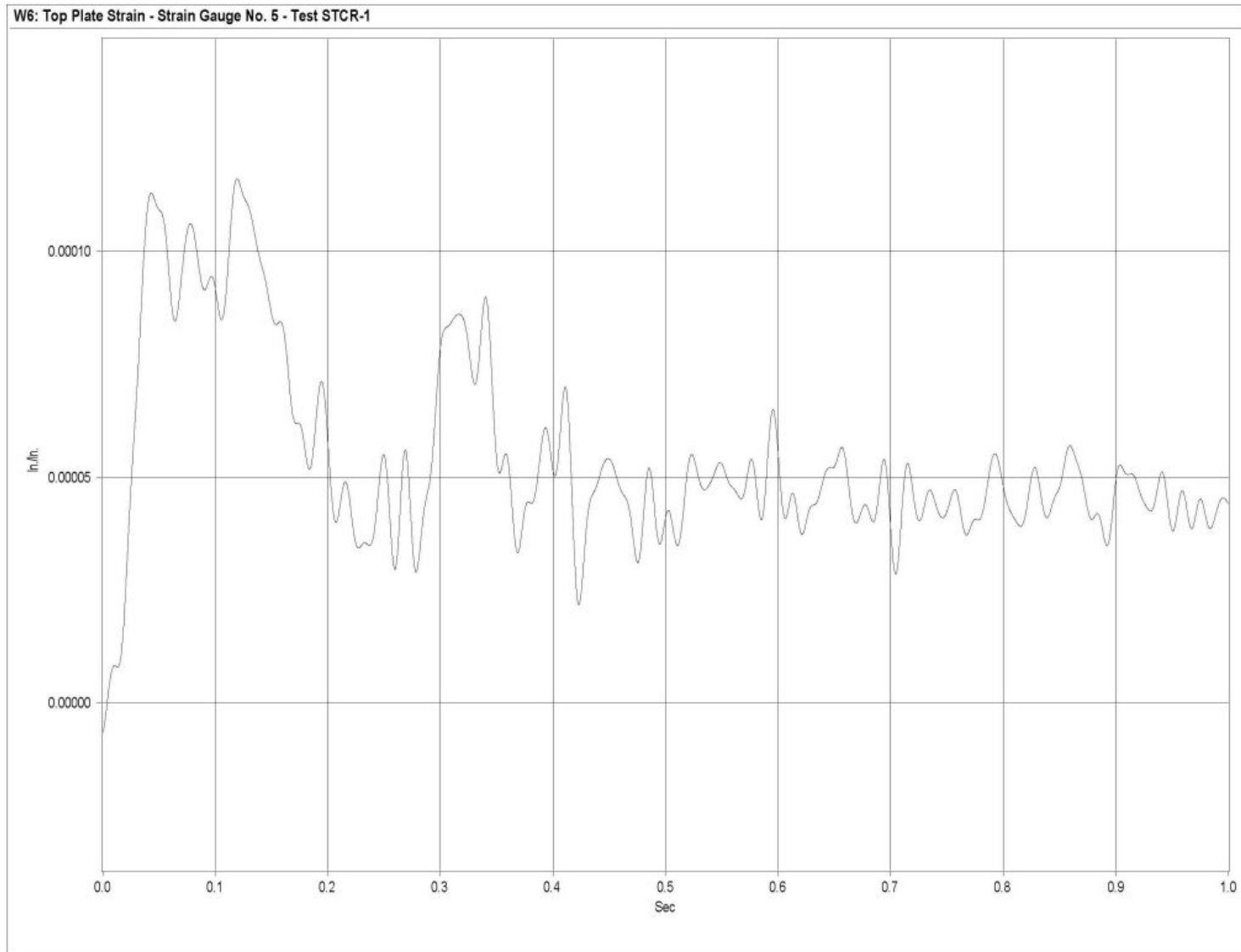
Figure G-9. Graph of Top Plate Post No. 5 - Strain Gauge No. 5 Perpendicular to Rail - Strain, Test STCR-1
