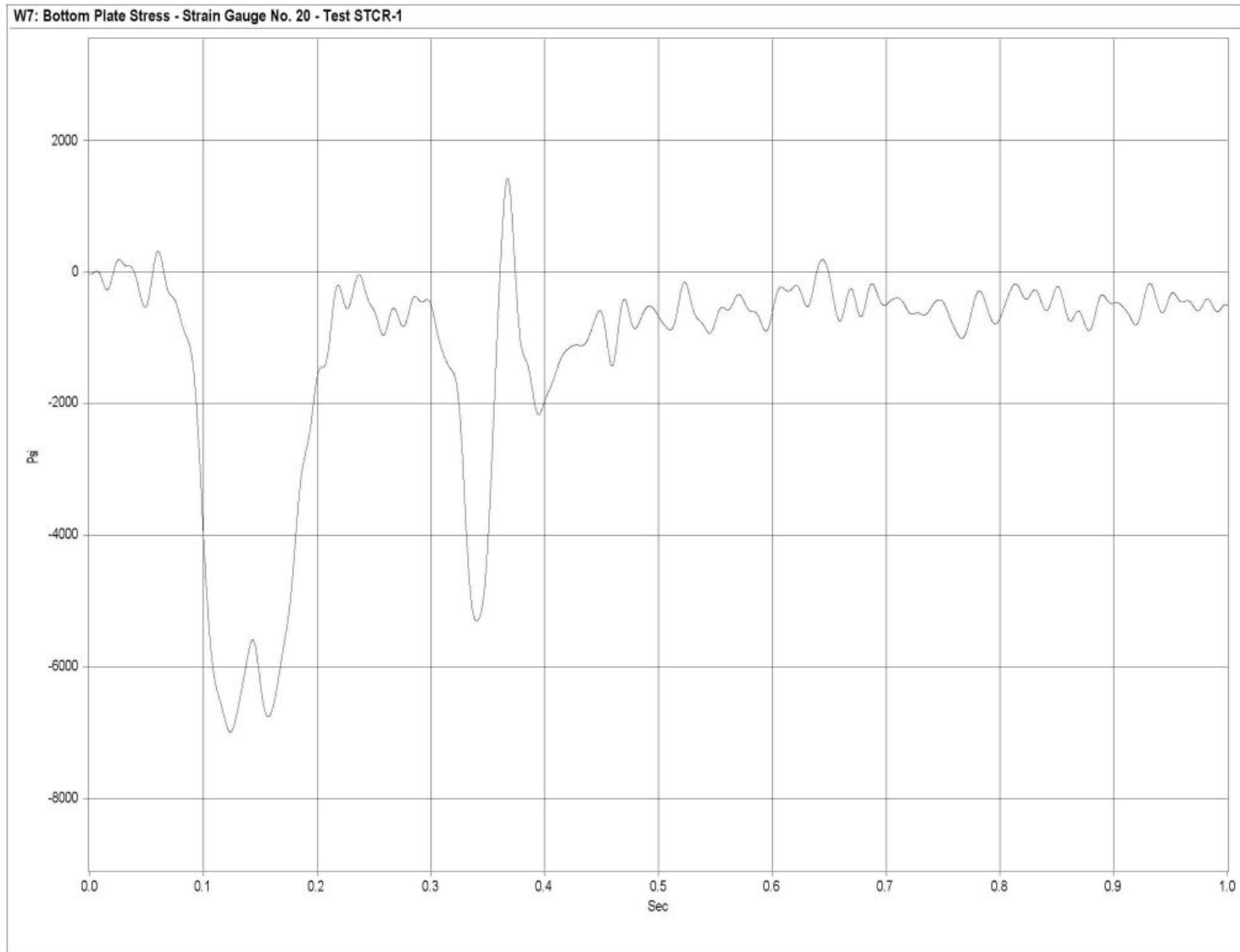
Figure G-35. Graph of Bottom Plate Post No. 7 - Strain Gauge No. 20 Perpendicular to Rail - Stress, Test STCR-1
