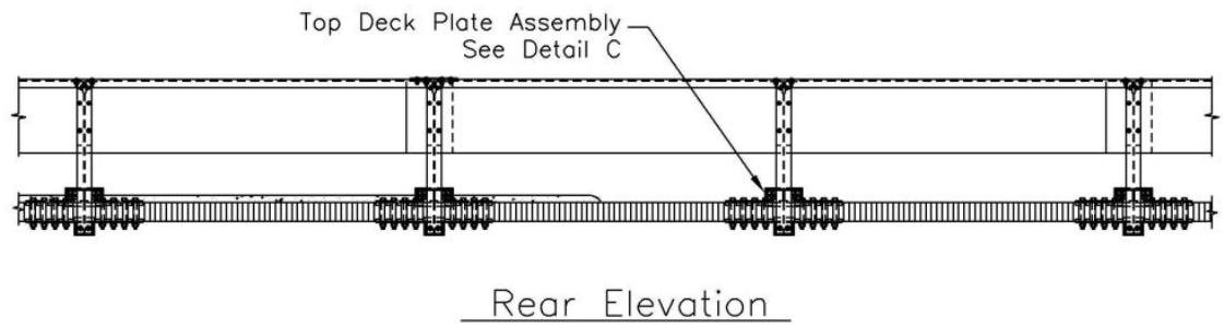
Figure 32. General Configuration of Steel Bridge Railing System
