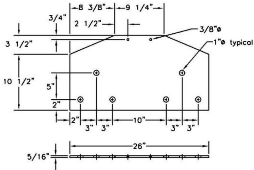
Deck Plates
