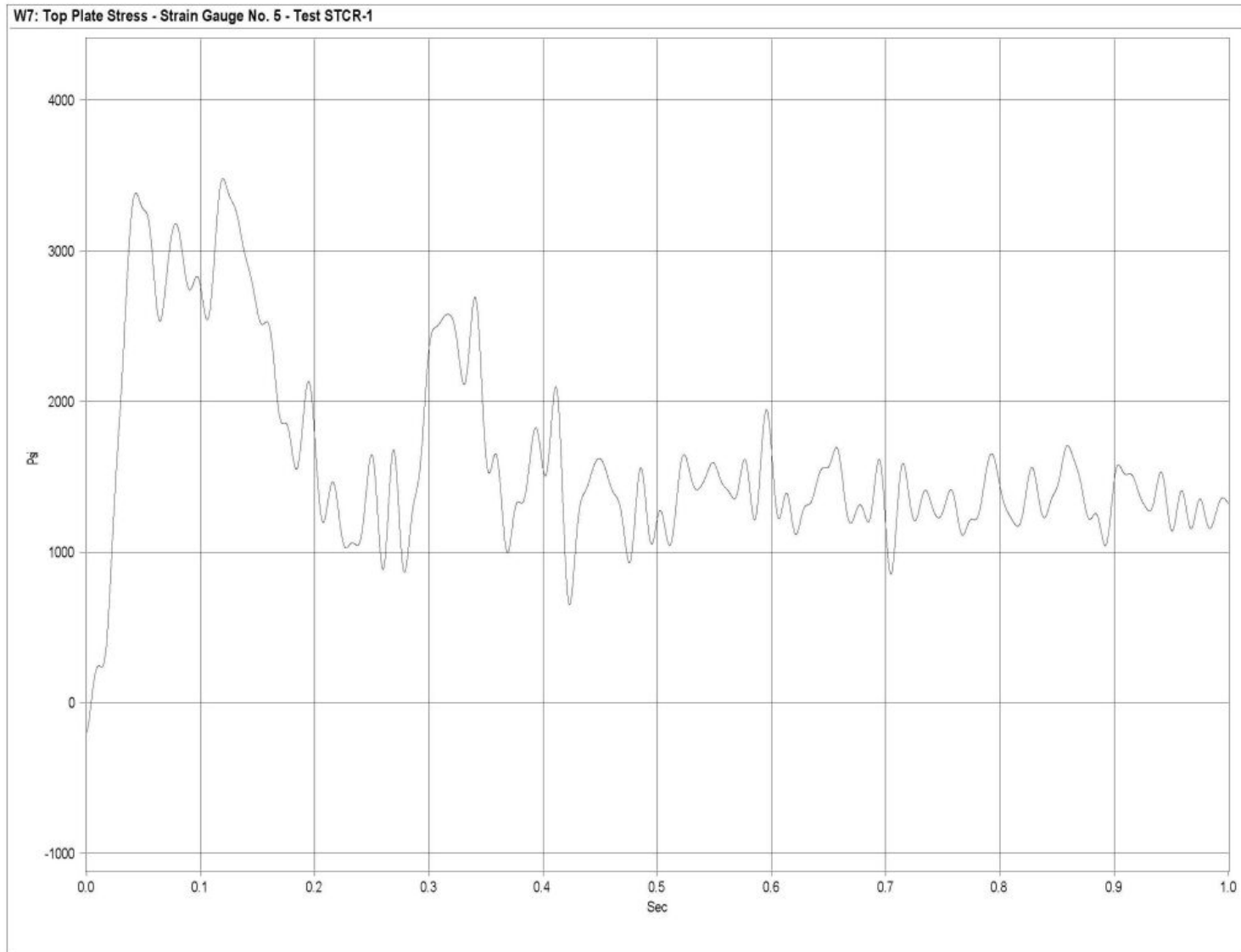
Figure G-10. Graph of Top Plate Post No. 5 - Strain Gauge No. 5 Perpendicular to Rail - Stress, Test STCR-1
