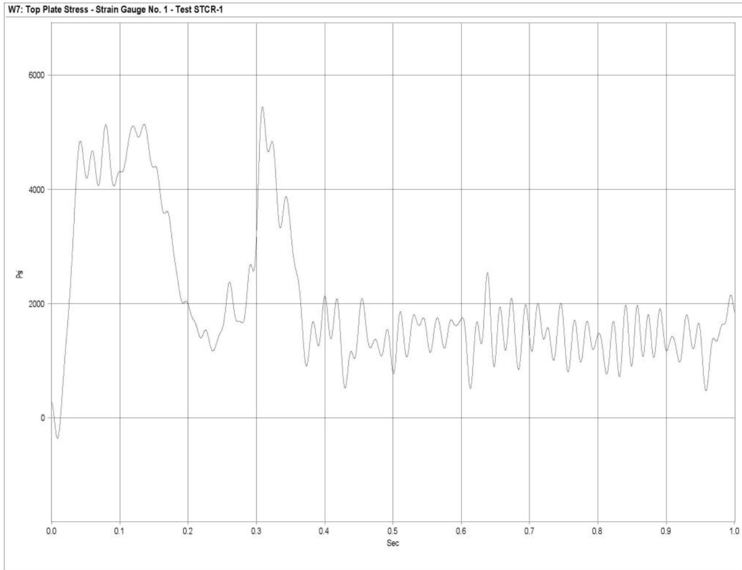
Figure G-2. Graph of Top Plate Post No. 5 - Strain Gauge No. 1 Perpendicular to Rail - Stress, Test STCR-1
