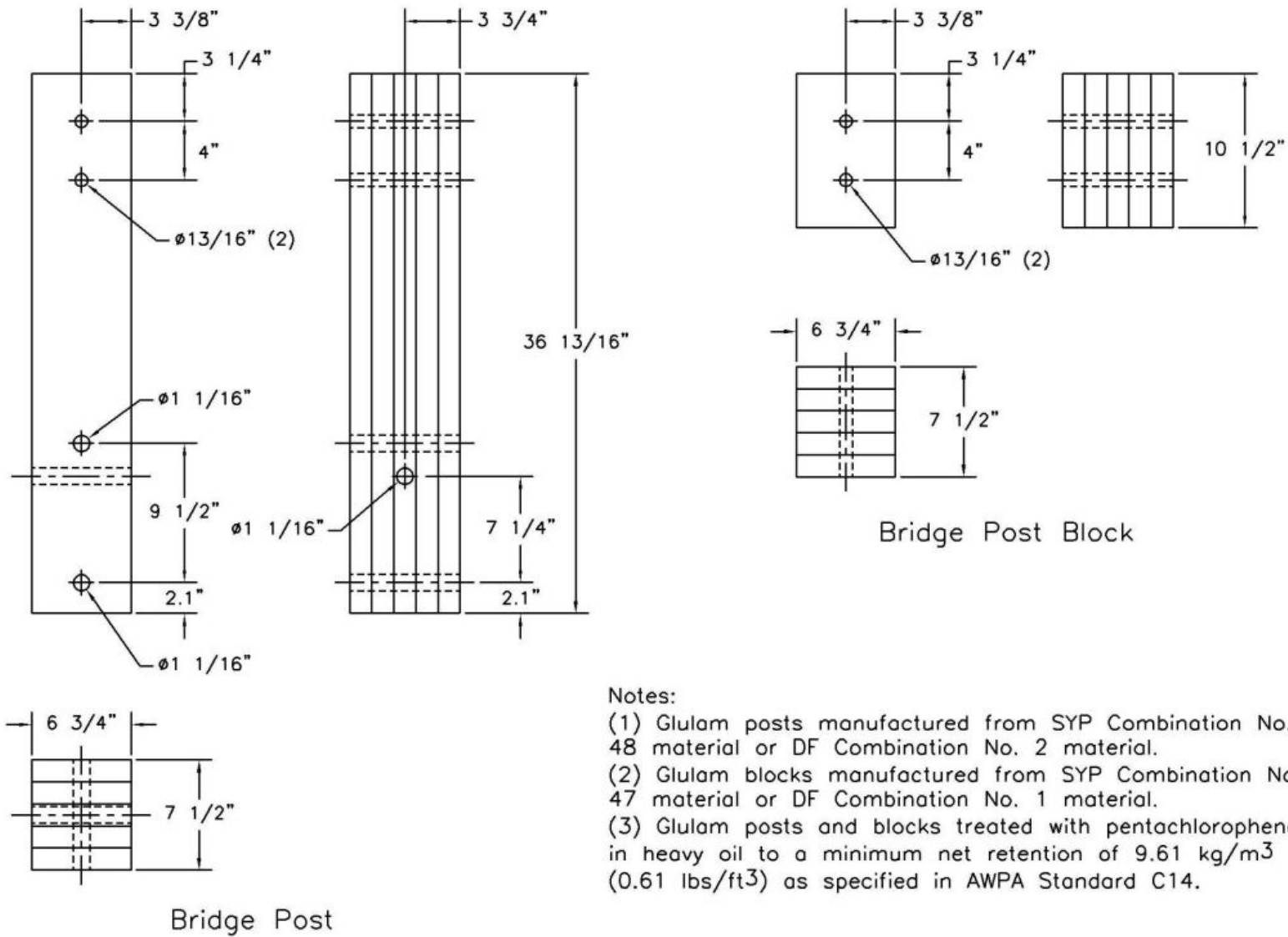
Figure 95. Bridge Post and Spacer Block Design Details
