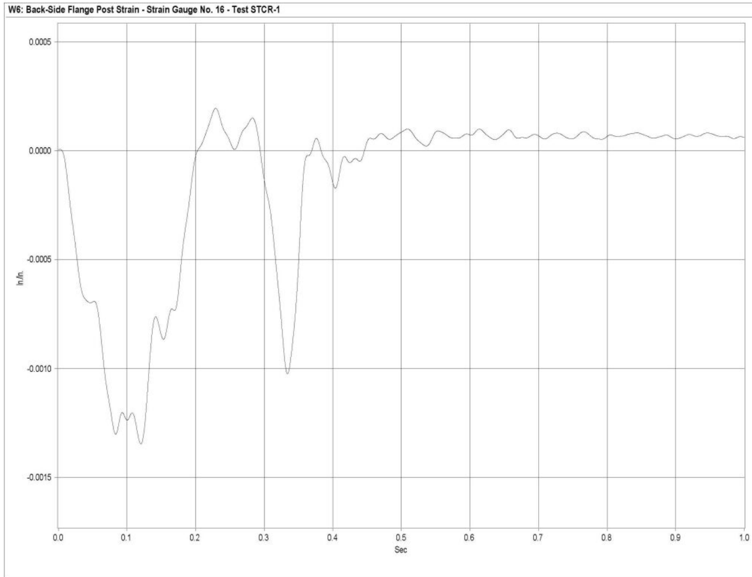
Figure G-26. Graph of Back-Side Flange Post No. 6 - Strain Gauge No. 16 - Strain, Test STCR-1
