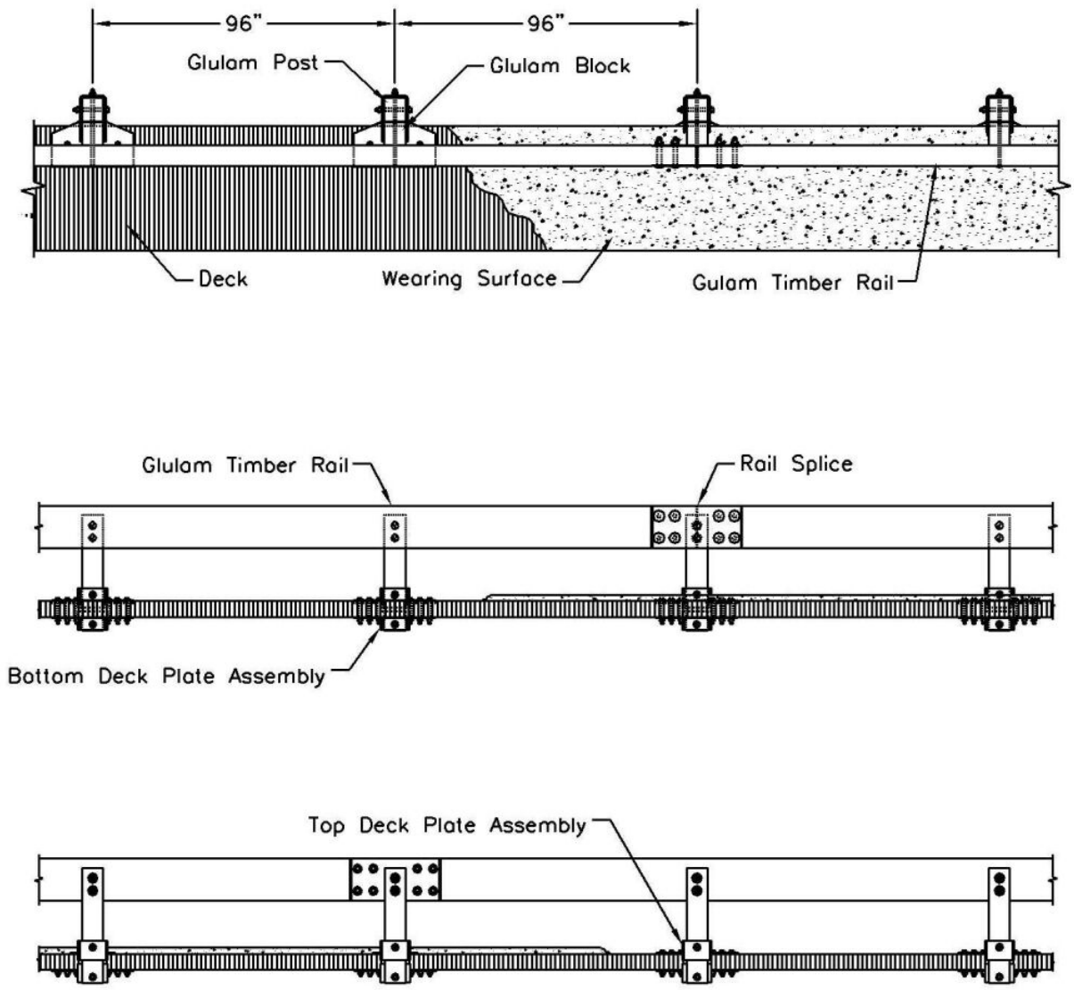
Figure 90. General Configuration of Wood Bridge Railing System
