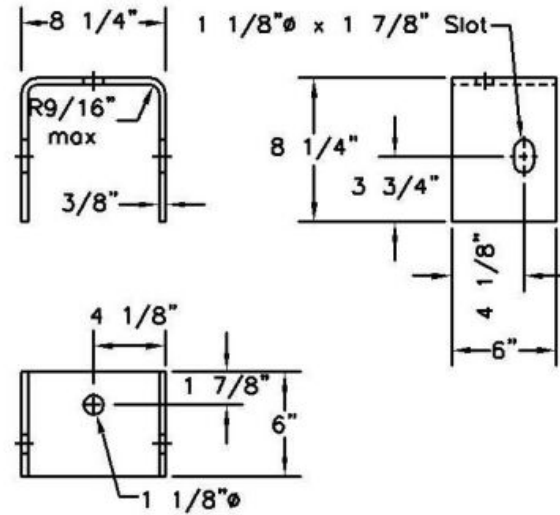
Bent Post Plates
