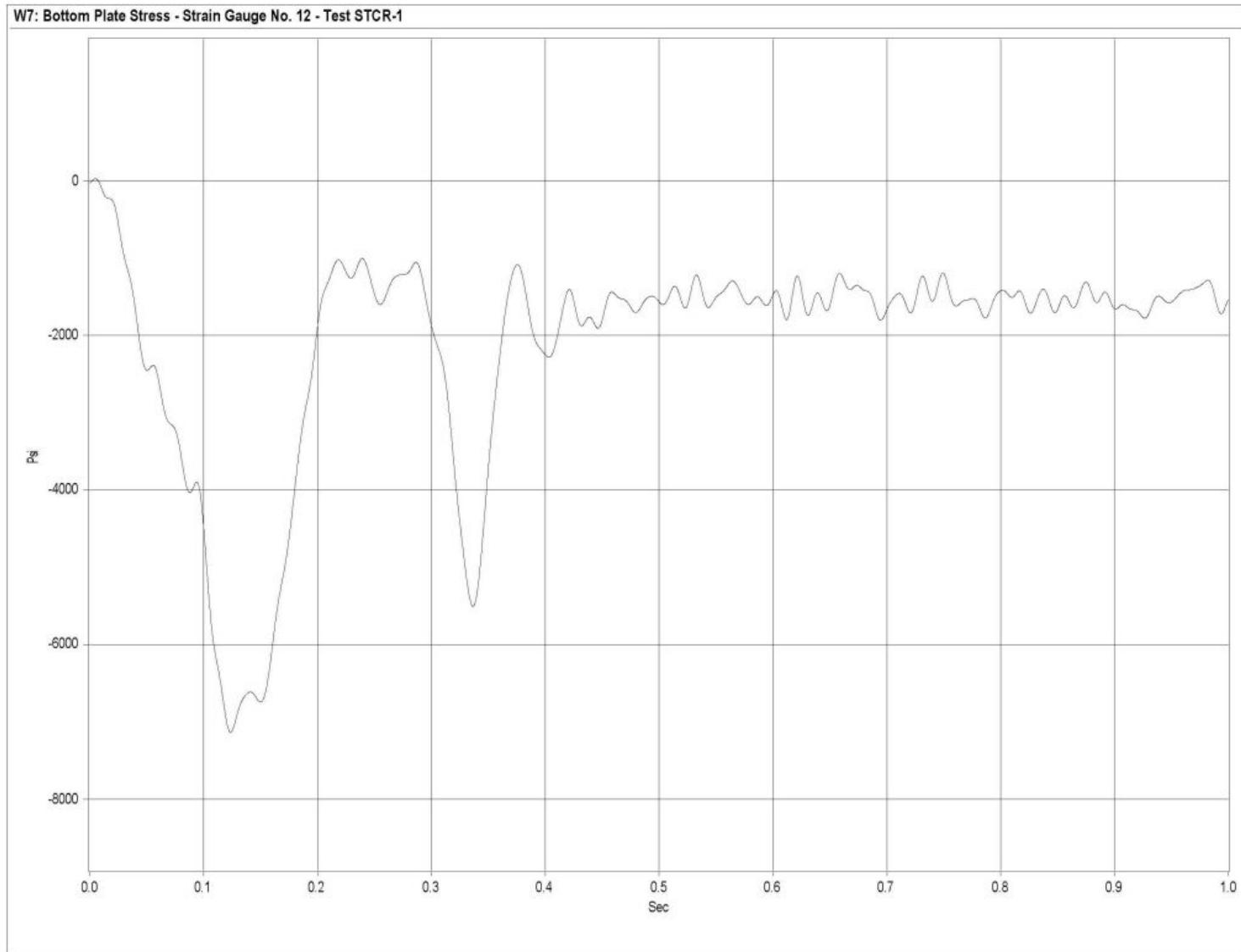
Figure G-20. Graph of Bottom Plate Post No. 6 - Strain Gauge No. 12 Perpendicular to Rail - Stress, Test STCR-1
