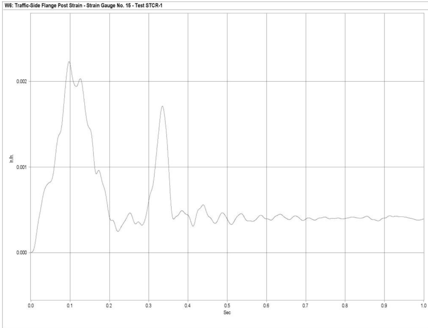
Figure G-25. Graph of Traffic-Side Flange Post No. 6 - Strain Gauge No. 15 - Strain, Test STCR-1
