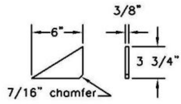
Plate Stiffener
