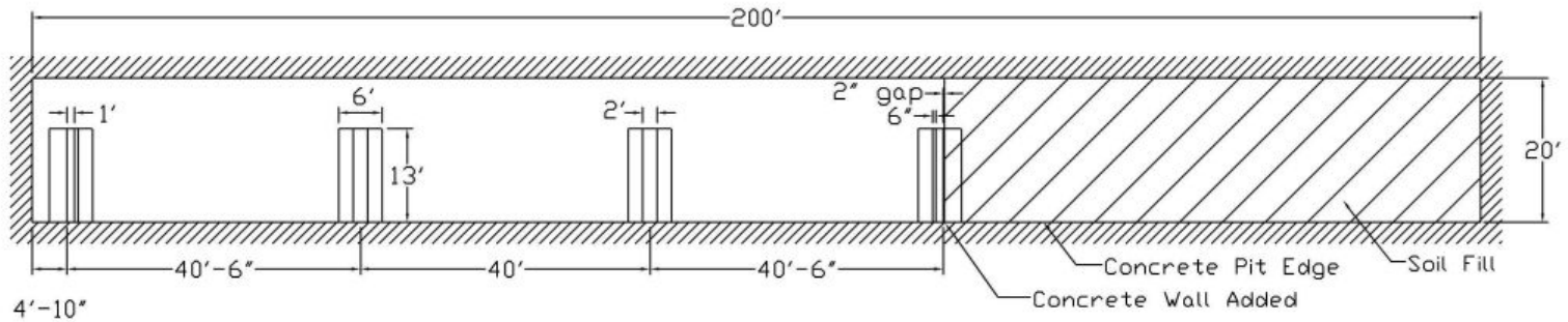
PLAN VIEW
