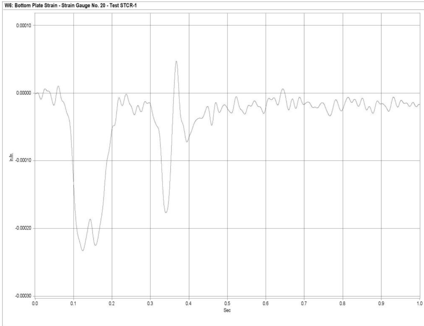
Figure G-34. Graph of Bottom Plate Post No. 7 - Strain Gauge No. 20 Perpendicular to Rail - Strain, Test STCR-1
