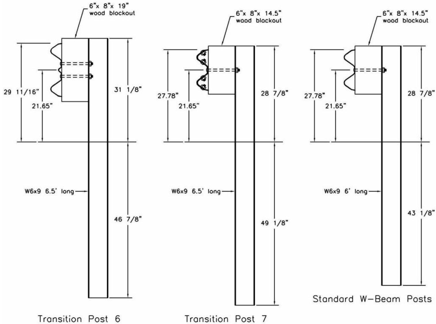
Figure 52. Transition Post Nos. 6 through 13 Configurations
