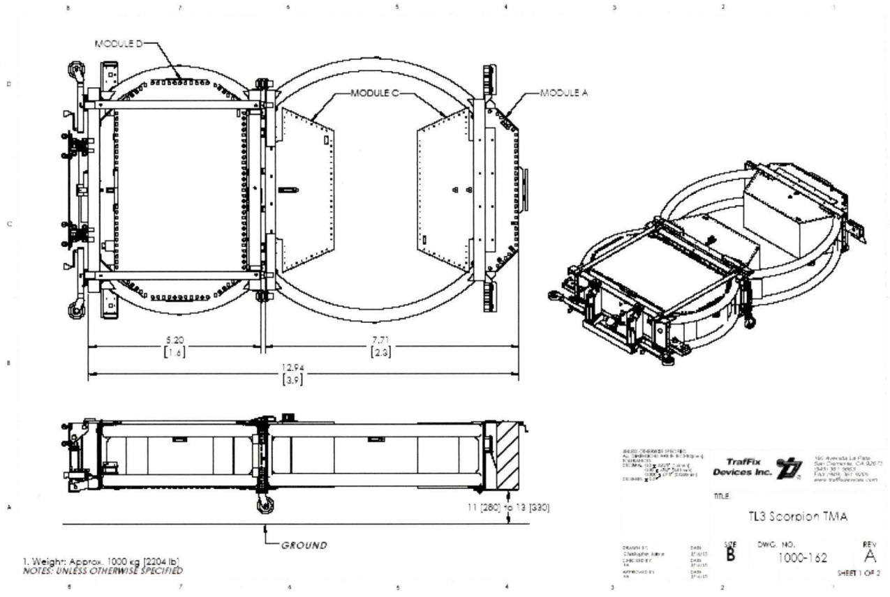
Figure 1: TL3 Scorpion TMA Sheet 1 of 2
