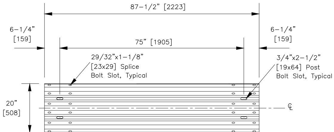
FRONT ELEVATION VIEW
