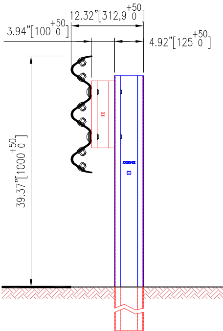
C-POST ELEVATION
