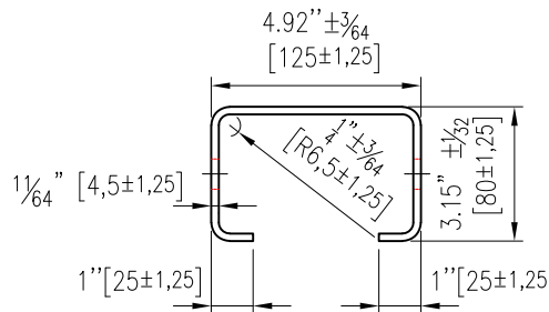
C-POST PLAN
