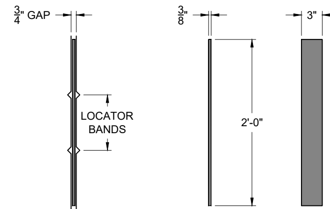
SPACER DETAIL
