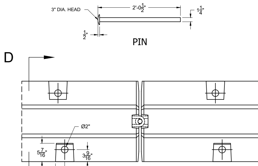
CONNECTION PLAN VIEW
