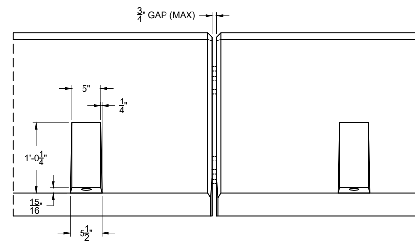
CONNECTION ELEVATION
